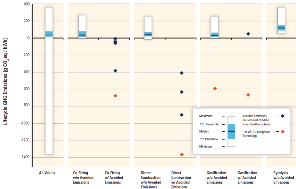
Figure 3. Life Cycle GHG Emission Estimates from Bio-Based Electricity Generation [Source: IPCC (2011)]
