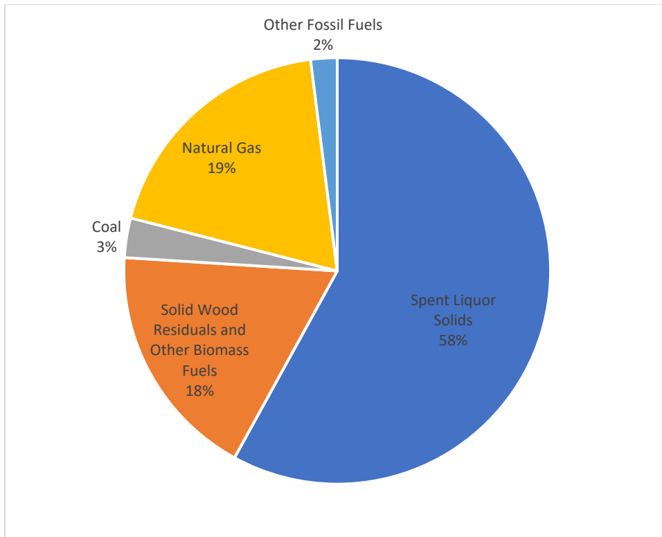
Figure 12. Fuels Used in US Pulp and Paper Sector Cogeneration Systems in 2018
